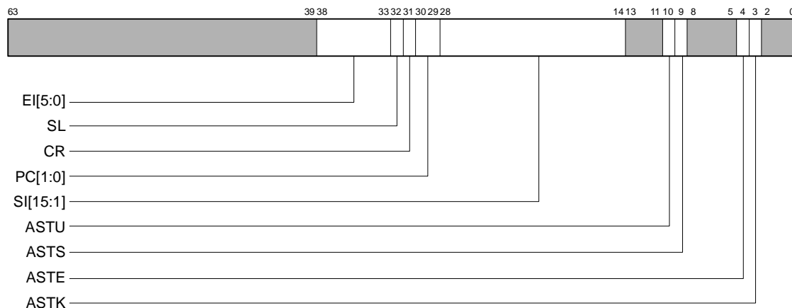
Figure 5–18 Interrupt Summary Register
