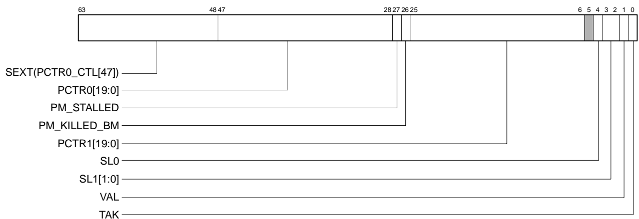
Figure 5–25 Performance Counter Control Register
