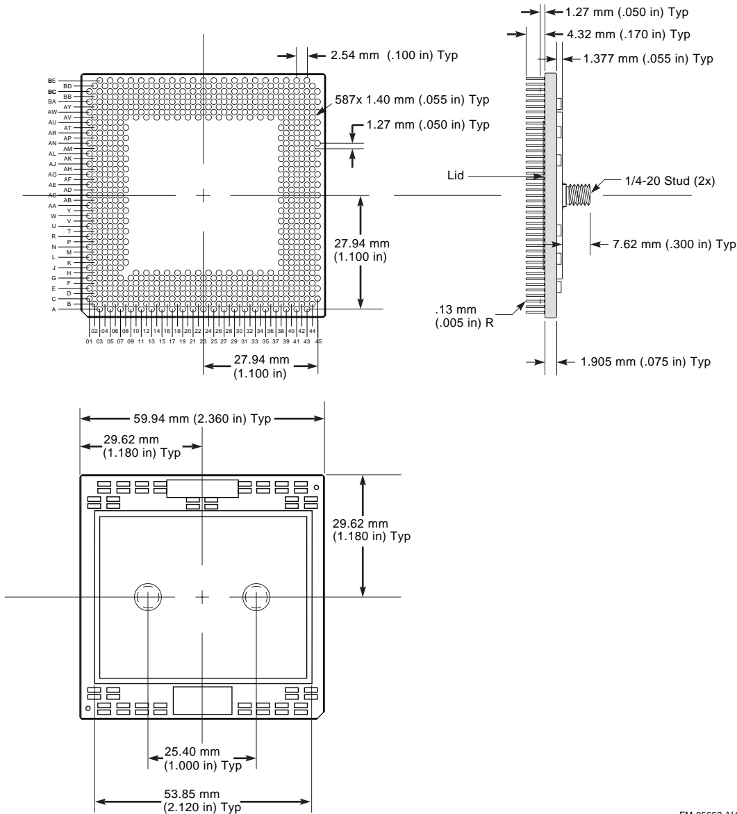
Figure 3–2 Package Dimensions
