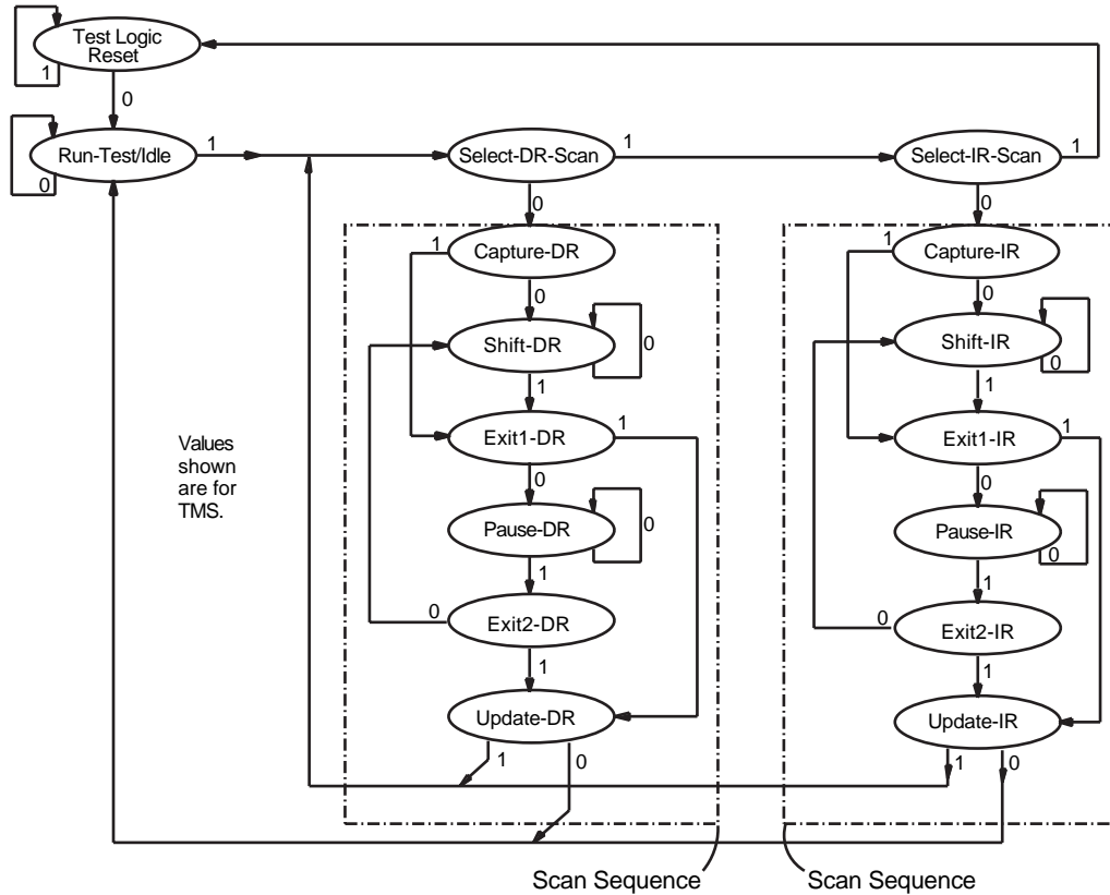
Figure 11–1 TAP Controller State Machine
