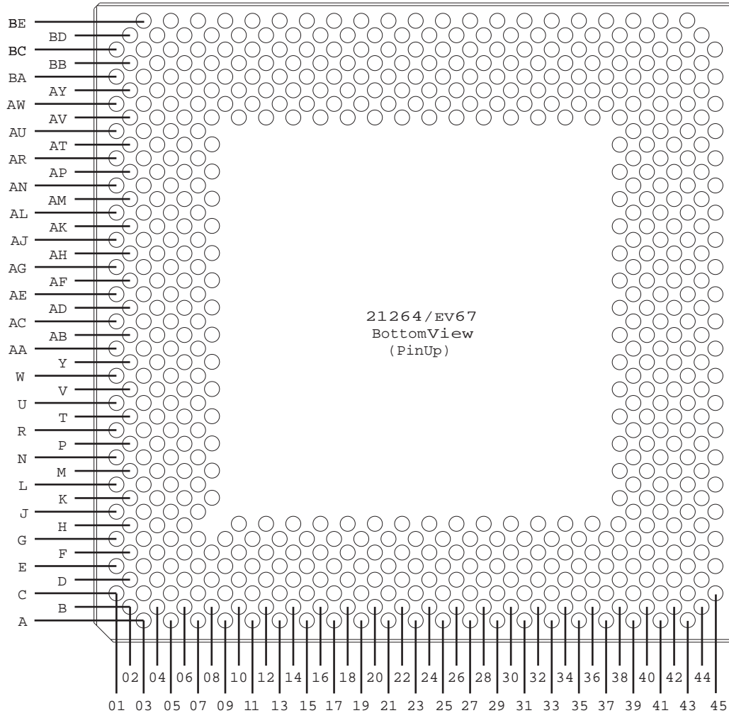
Figure 3-4 21264/EV67 Bottom View (Pin Up)
