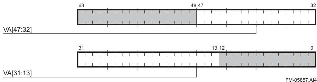
Figure 5–25 DTB Tag Array Write Registers 0 and 1
