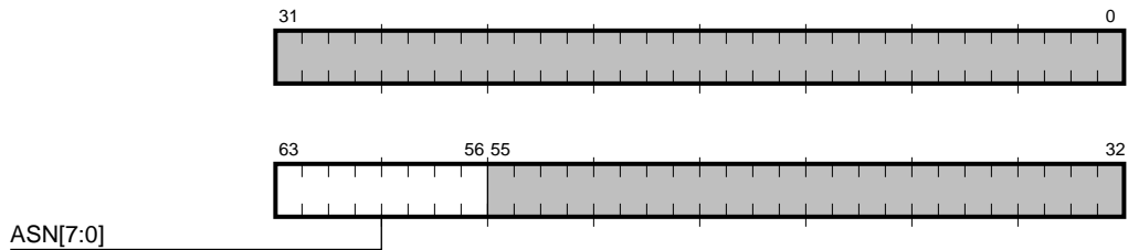
Figure 5–29 Dstream Translation Buffer Address Space Number Registers 0 and 1
