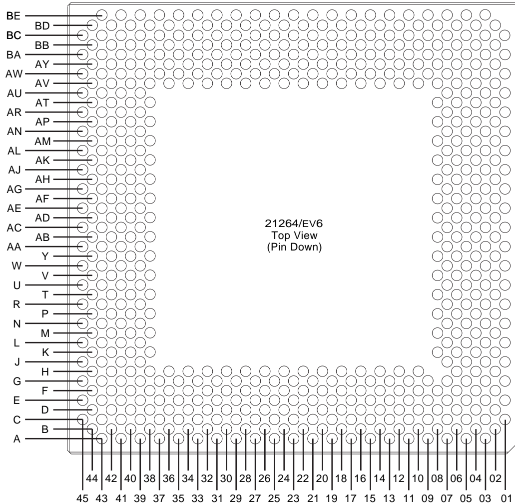
Figure 3-3 21264/EV6 Top View (Pin Down)
