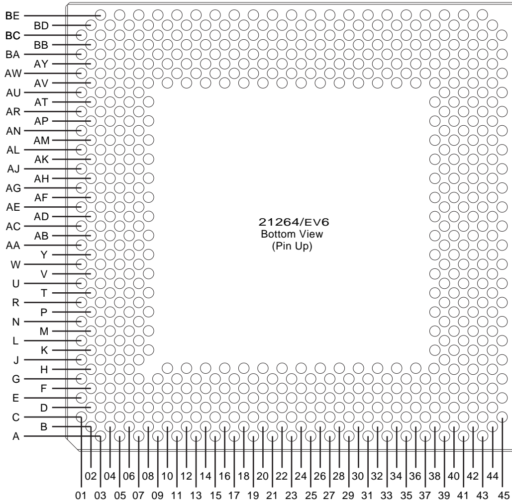
Figure 3-4 21264/EV6 Bottom View (Pin Up)
