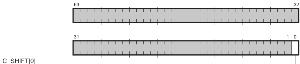
Figure 5–35 Cbox Shift Register
