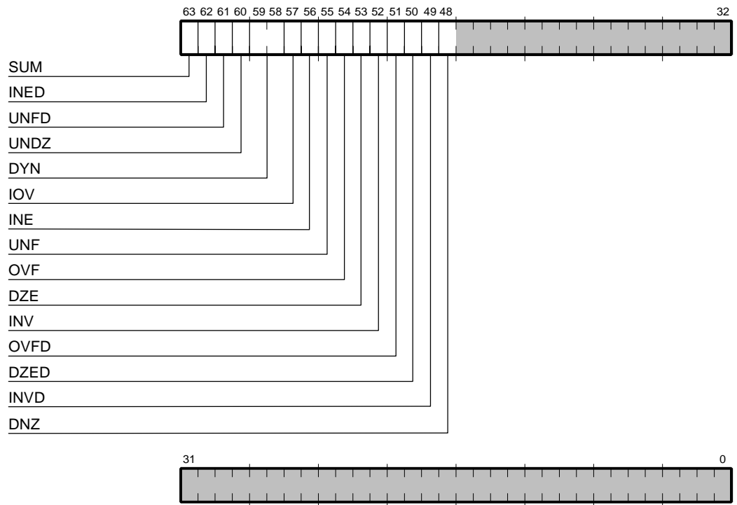
Figure 2–11 Floating-Point Control Register
