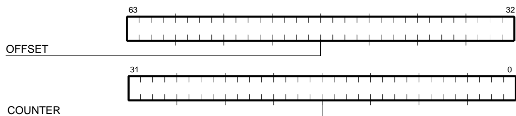
Figure 5–1 Cycle Counter Register
