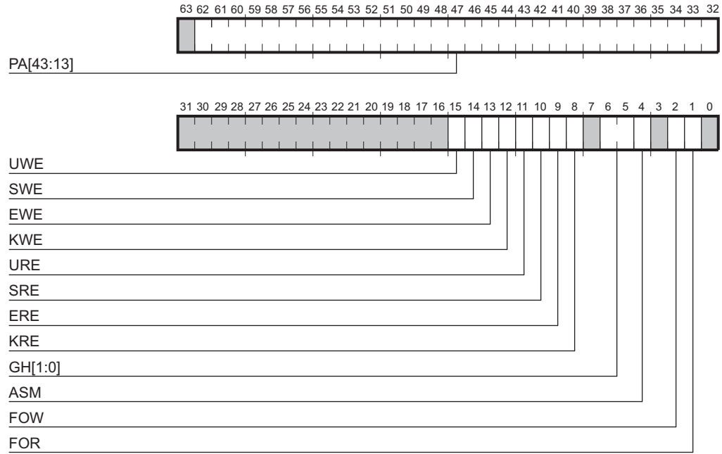
Figure 5–26 DTB PTE Array Write Registers 0 and 1
