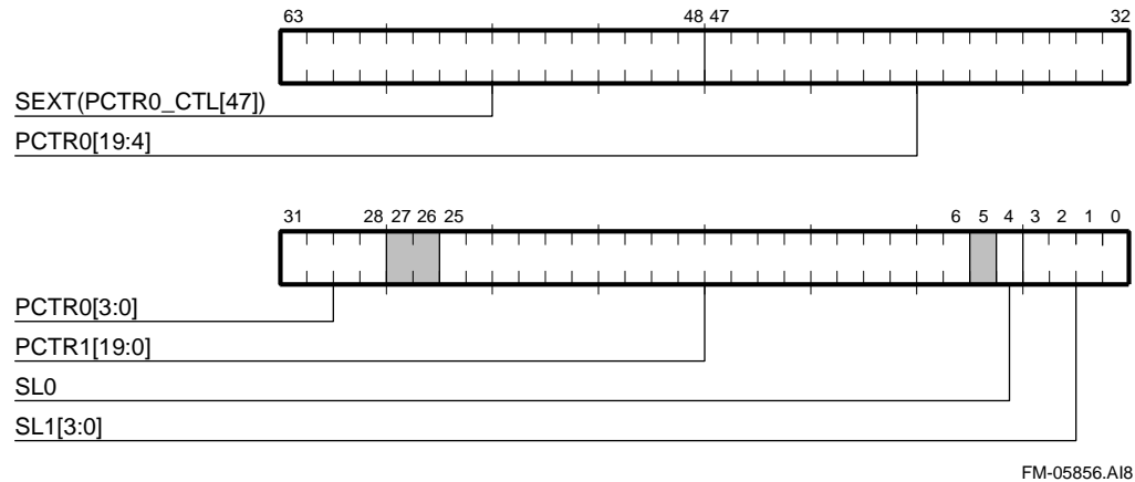
Figure 5–24 Performance Counter Control Register
