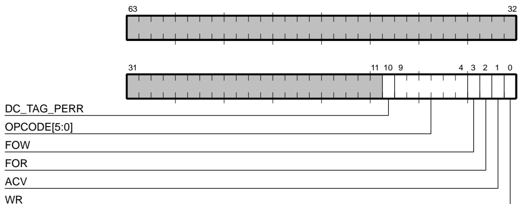
Figure 5–30 Memory Management Status Register
