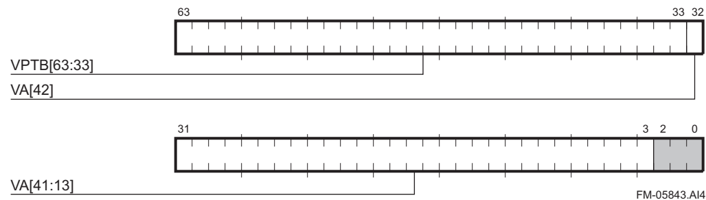
Figure 5–12 Instruction Virtual Address Format Register (VA_48 = 0, VA_FORM_32 = 0)
