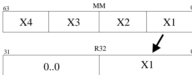
Example 4-15 pextrw Instruction Code
