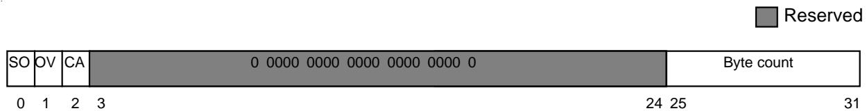
Figure 2-5. XER Register
