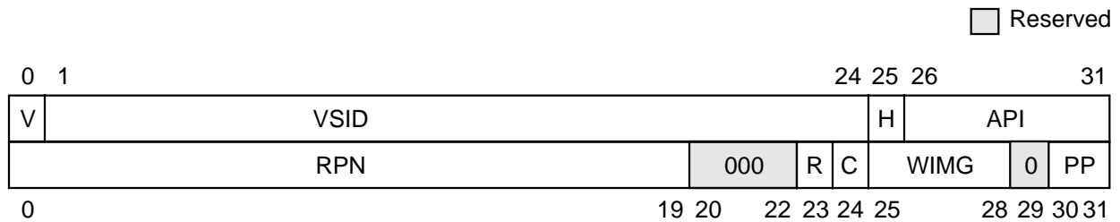
Figure 7-14. Page Table Entry Format
