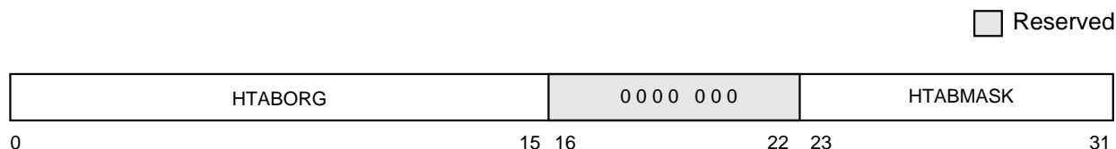
Figure 7-19. SDR1 Register Format
