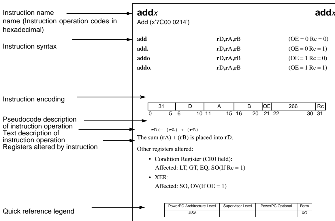
Figure 8-1. Instruction Description
