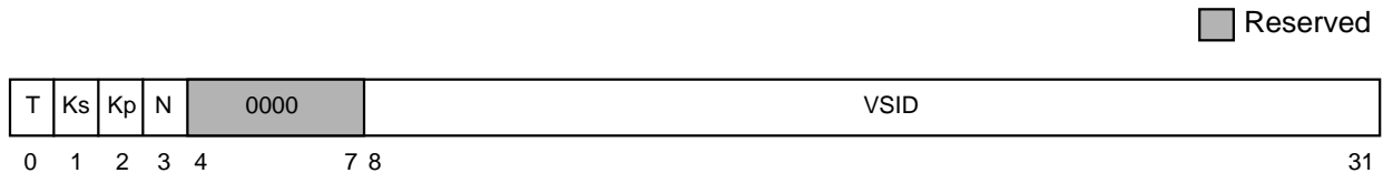
Figure 2-16. Segment Register Format ( T = 0 )
