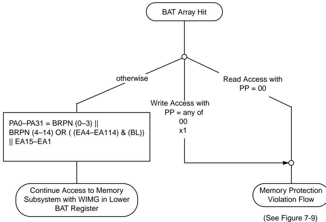
Figure 7-11. Block Address Translation Flow
