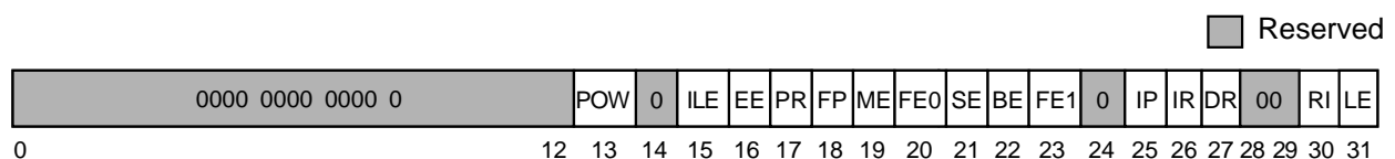
Figure 2-11. Machine State Register (MSR)
