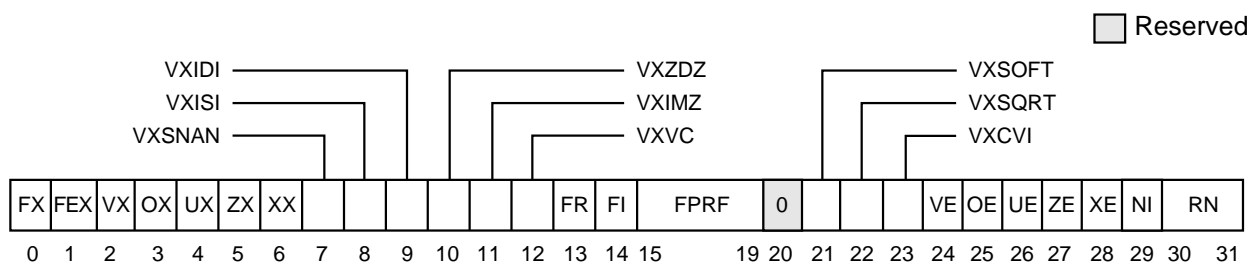
Figure 3-22. Floating-Point Status and Control Register (FPSCR)
