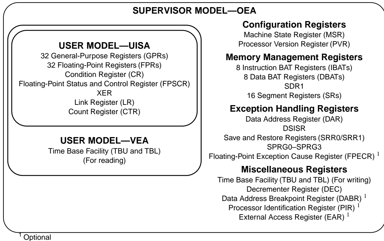
Figure 1-1. Programming Model—PowerPC Registers
