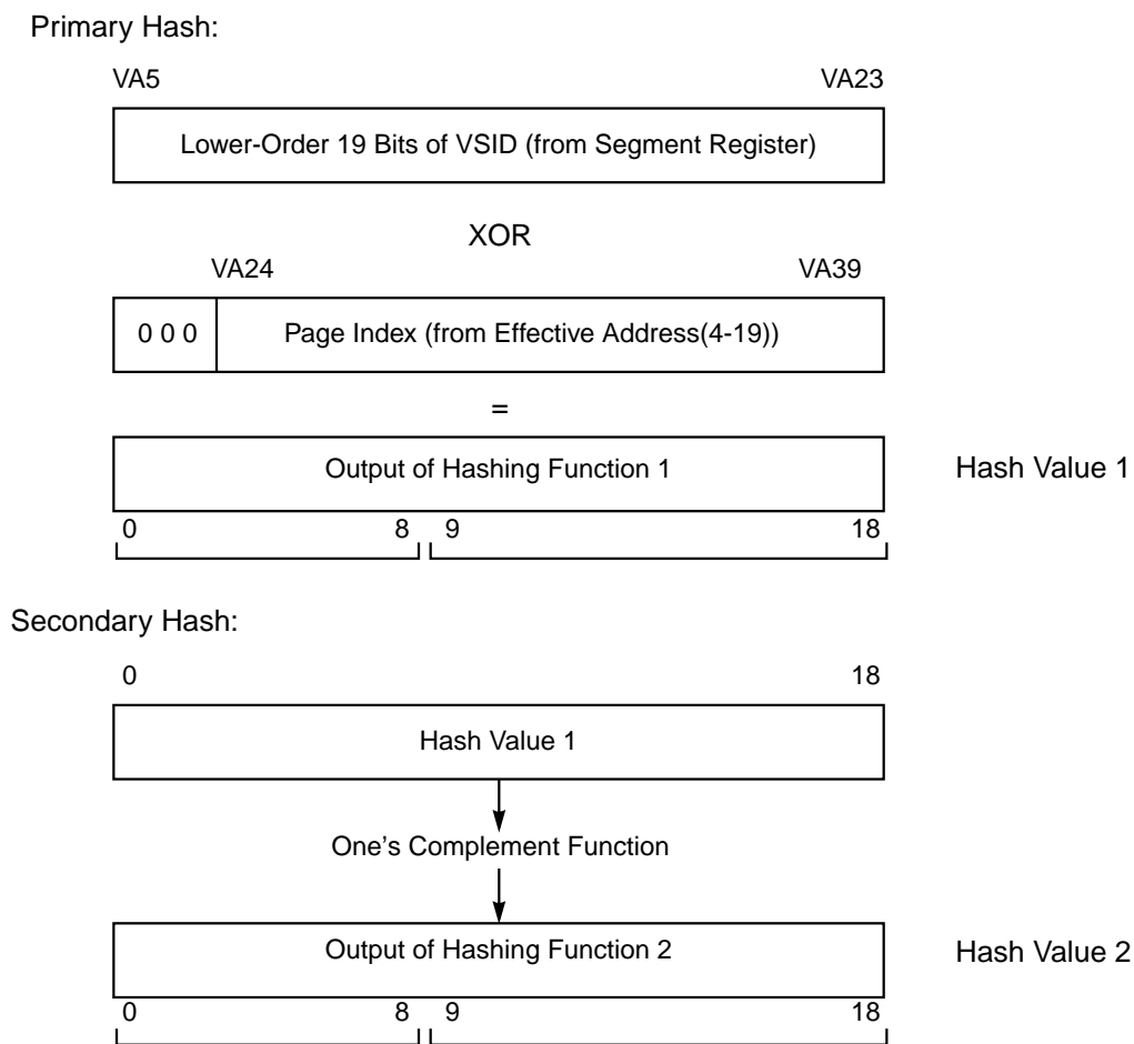
Figure 7-20. Hashing Functions for Page Tables
