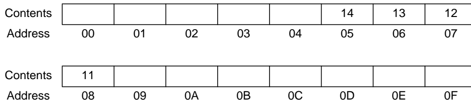
Figure 3-7. True Little-Endian Mapping, Word Stored at Address 05
