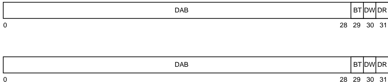
Figure 2-24. Data Address Breakpoint Register (DABR)
