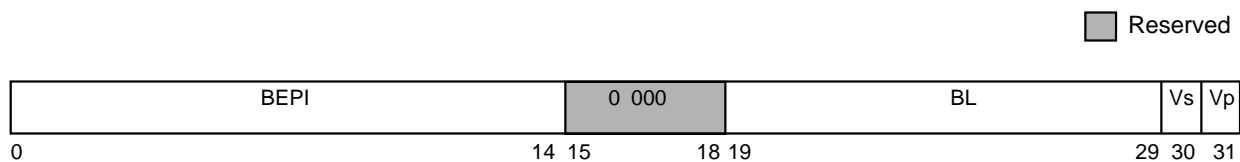
Figure 2-13. Upper BAT Register
