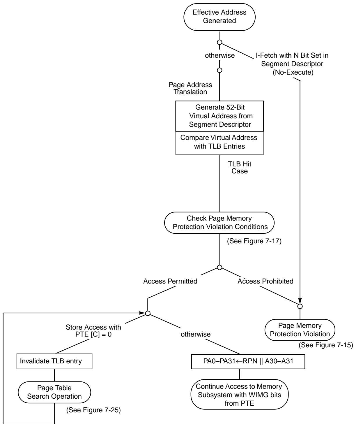
Figure 7-16. Page Address Translation Flow—TLB Hit
