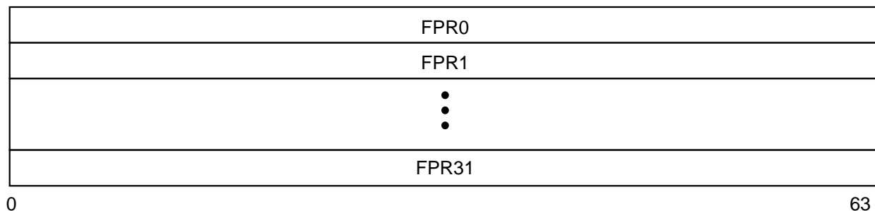
Figure 2-2. Floating-Point Registers (FPRs)
