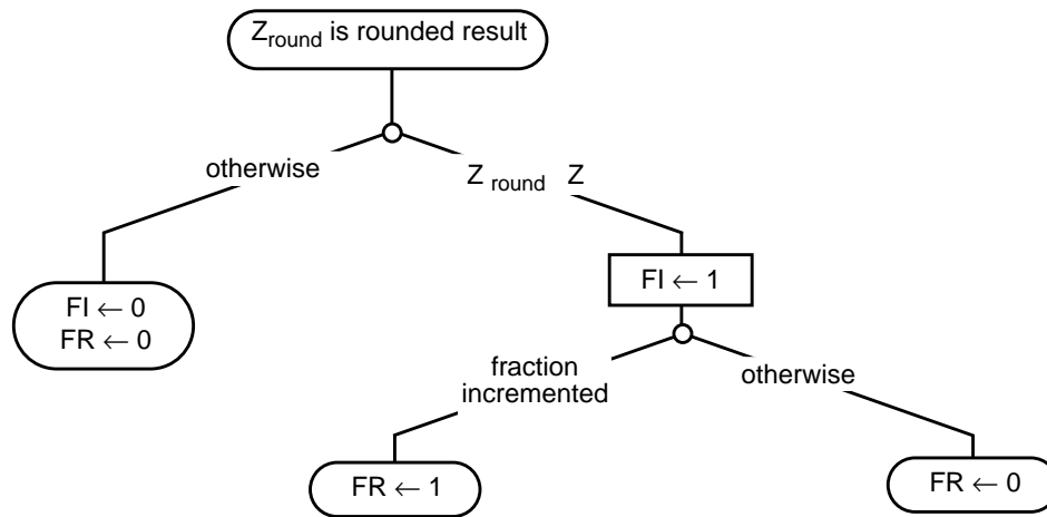
Figure 3-21. Rounding Flags in FPSCR
