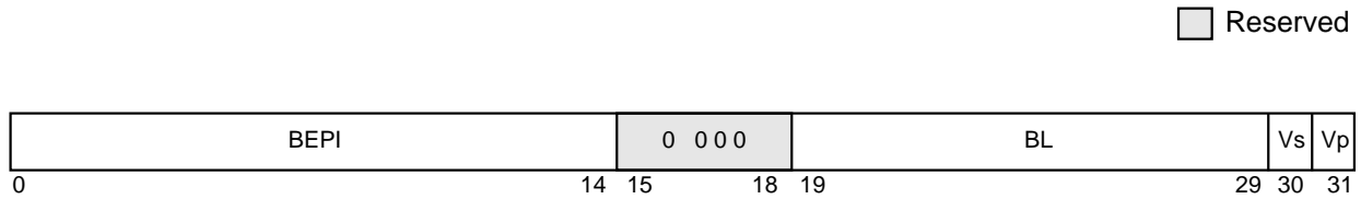
Figure 7-7. Format of Upper BAT Registers
