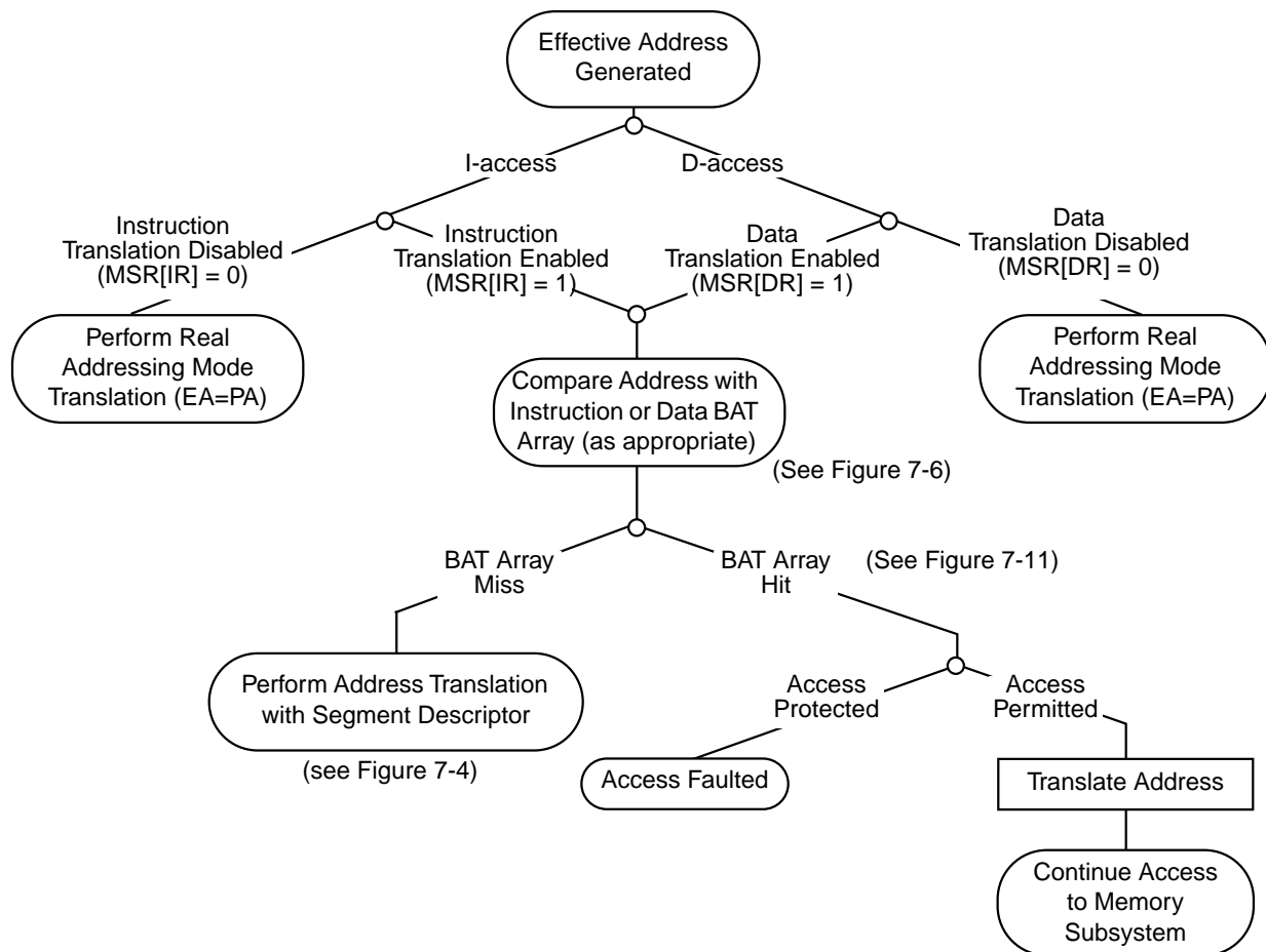
Figure 7-3. General Flow of Address Translation
