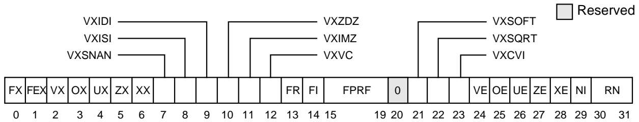
Figure 2-4. Floating-Point Status and Control Register (FPSCR)
