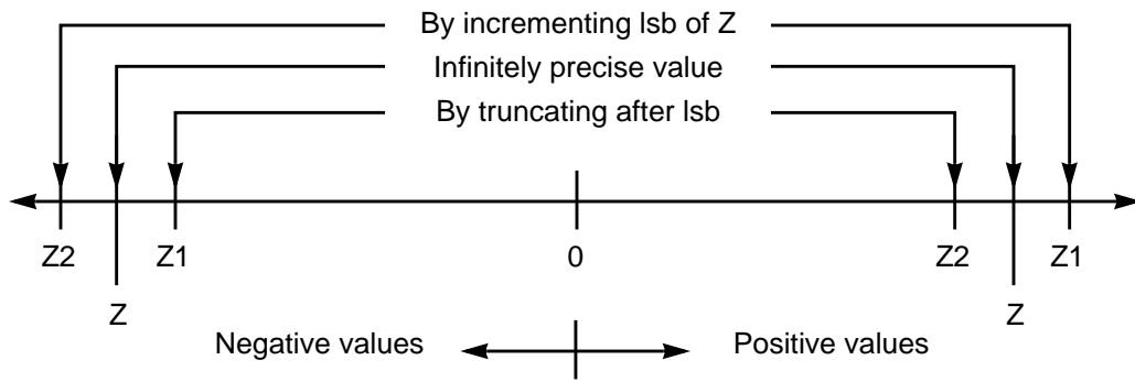
Figure 3-19. Relation of Z1 and Z2
