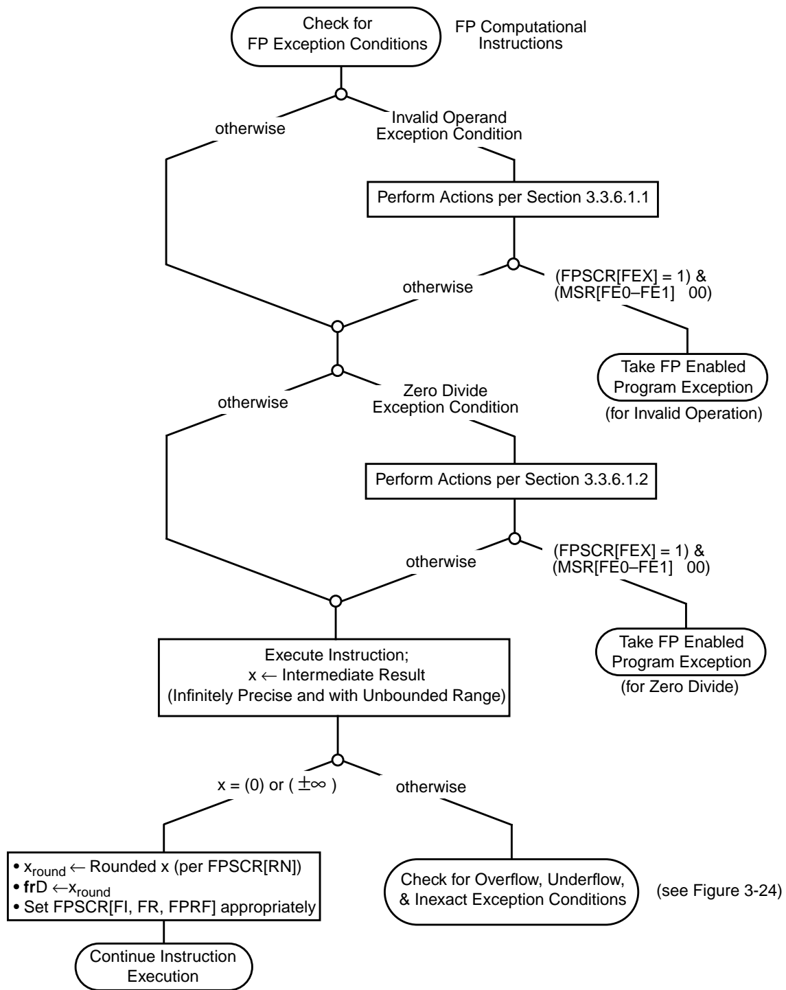
Figure 3-23. Initial Flow for Floating-Point Exception Conditions
