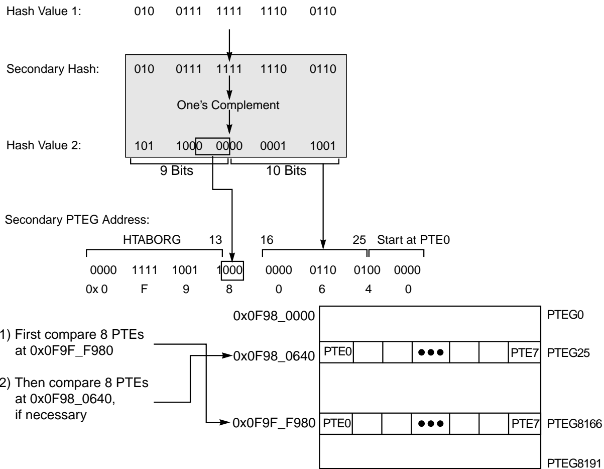
Figure 7-24. Example Secondary PTEG Address Generation
