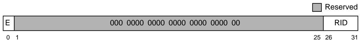
Figure 2-25. External Access Register (EAR)
