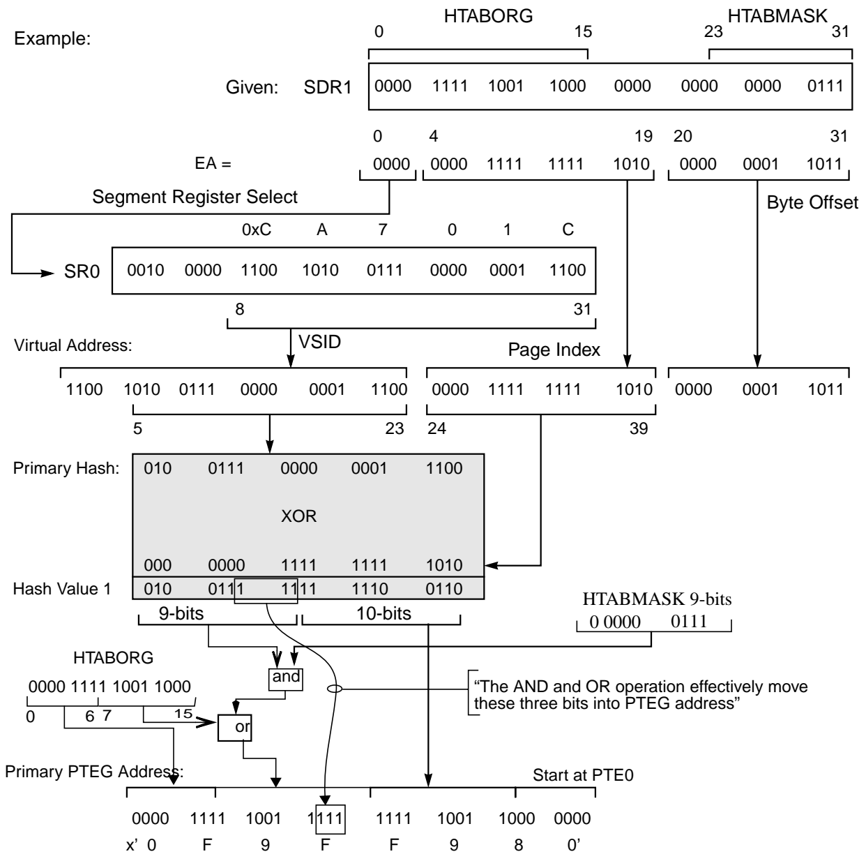
Figure 7-23. Example Primary PTEG Address Generation
